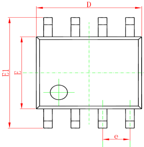
SOP-8L PACKAGE DIAGRAMS TOP VIEW
