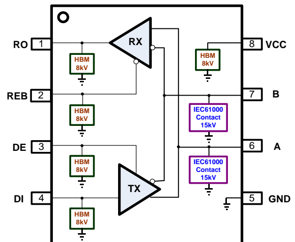
Functional Block of AZRS3080E
