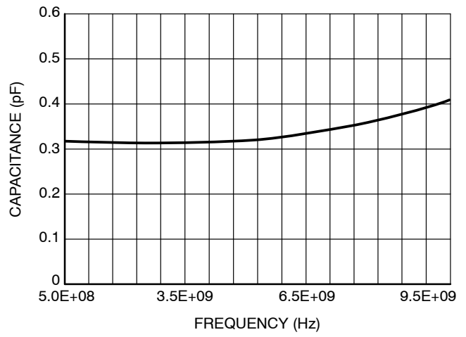
Figure 10. Junction Capacitance; V R = 0 V, f = 500 MHz – 10 GHz
