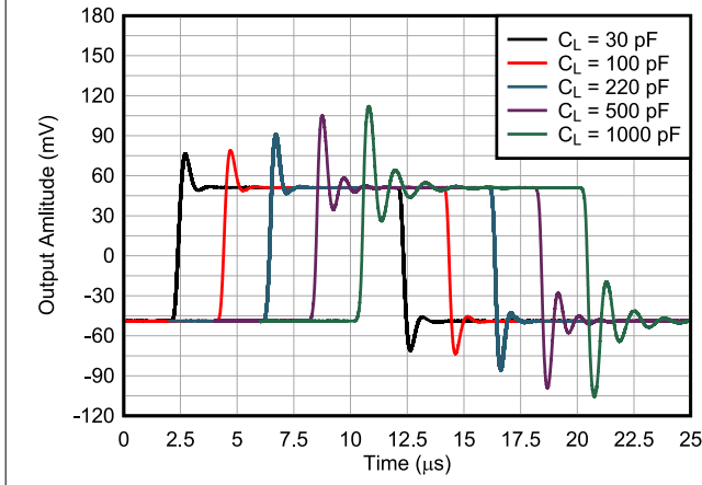
Figure 7-33. Overshoot vs Capacitive Loads
