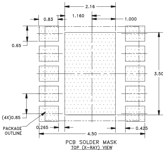
Figure 4: PCB Footprint
