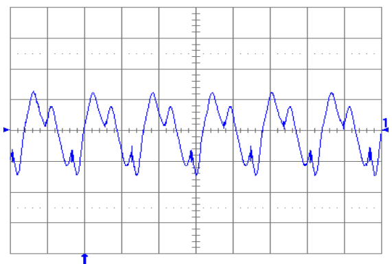
Fig. 5.0V.6: Output voltage ripple (10mV/div.) at full rated load current into a resistive load with external capacitance 47\mu\text{F} ceramic + 1\mu\text{F} ceramic and V_{in} = 12V for V_{out} = 5.0V . Time scale: 2 \mu\text{s}/\text{div} .
