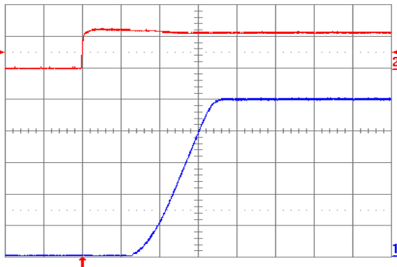
Fig. 5.0V.5: Turn-on transient for V_{out} = 5.0V with application of V_{in} at full rated load current (resistive) and 47\mu\text{F} external capacitance at V_{in} = 12V . Top trace: V_{in} (10V/div.); Bottom trace: output voltage (1V/div.); Time scale: 5 ms/div.
