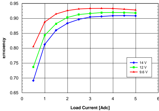
Fig. 5.0V.3: Efficiency vs. load current and input voltage for V_{out} = 5.0V converter mounted vertically with air flowing from pin 5 to pin 1 at a rate of 200 LFM (1 m/s) and T_a = 25^{\circ}\text{C} .
