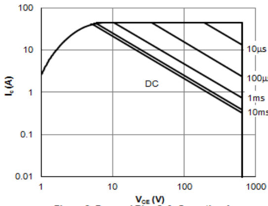
Figure 9: Forward Bias Safe Operating Area ( T_c=25^\circ C , V_{GE}=15V )
