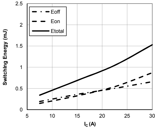
Figure 17: Switching Loss vs. I_C ( T_J=175^\circ\text{C} , V_{GE}=15\text{V} , V_{CE}=400\text{V} , R_\theta=20\Omega )
