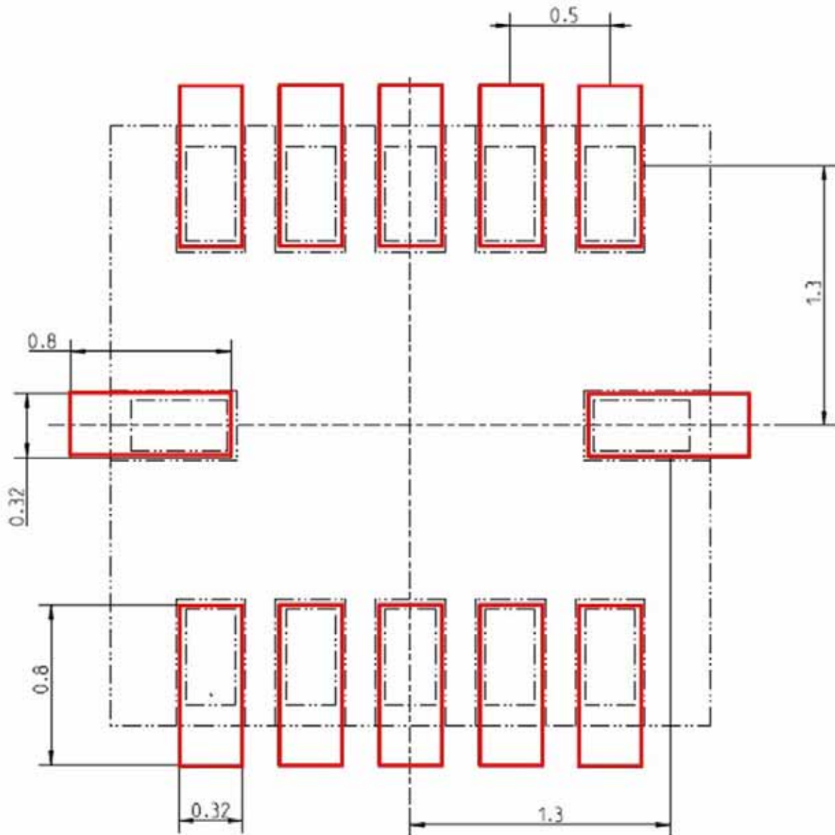
Figure 19: Landing patterns for the BMA150 relative to the device pins, dimensions are in mm
