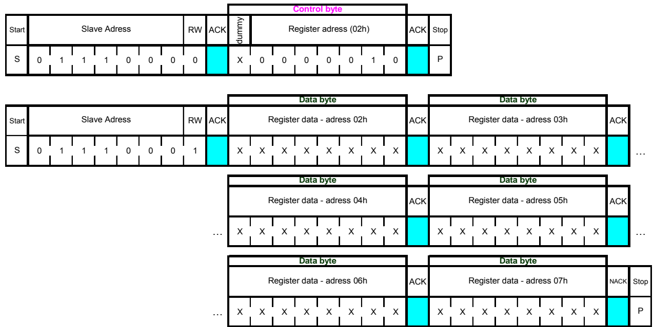
Figure 16: I 2 C multiple read protocol. Address register is first written to BMA150, the RW=0 (lowest acceleration data located at address 02h). I 2 C transfer is stopped and restarted with RW=1, address is automatically incremented and the 6 bytes can be sequentially read out.
