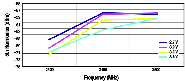
Figure 12. Fifth Harmonics vs Frequency Over Voltage (High Power Mode)
