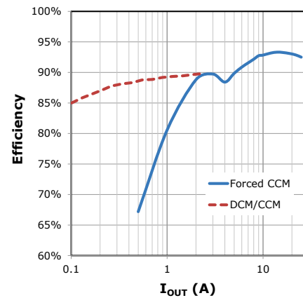
Fig. 15: Efficiency, 12V IN , 3.3V OUT , 1µH, 300kHz
