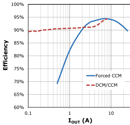
Fig. 12: Efficiency, 5V IN , 1.8V OUT , 0.47µH, 300kHz
