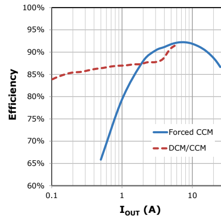
Fig. 13: Efficiency, 5V IN , 1.2V OUT , 0.47µH, 300kHz
