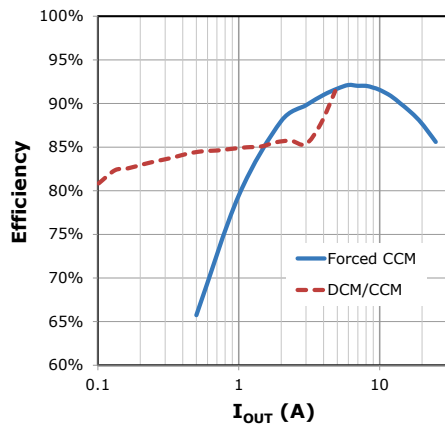
Fig. 14: Efficiency, 5V IN , 1.0V OUT , 0.47µH, 300kHz
