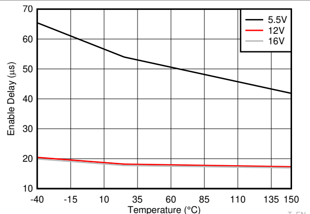
Figure 6-12. Enable Delay
