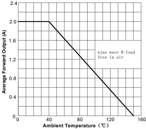
FIG1:Io-Ta Curve
