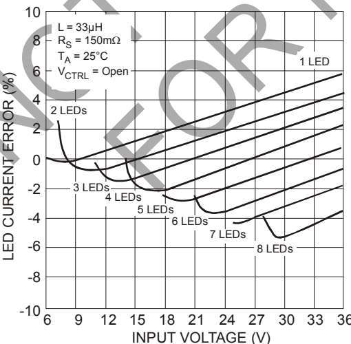
Figure 17. LED Current Deviation vs. Input Voltage
