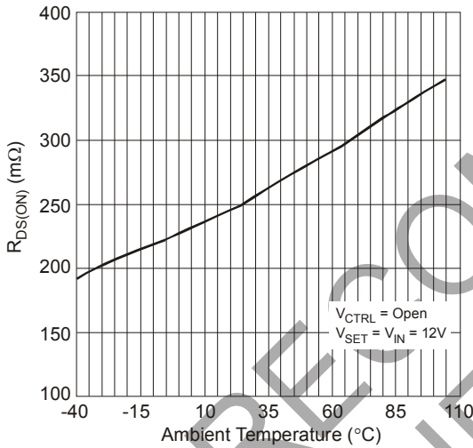
Figure 9. SW R_{DS(ON)} vs. Temperature
