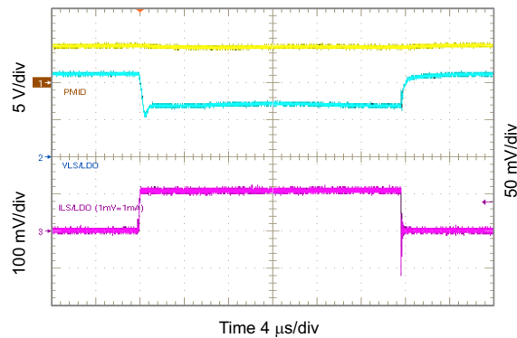
Figure 10-53. 1.2 V_{\text{LSLDO}} Load Transient, 0 to 100 mA
