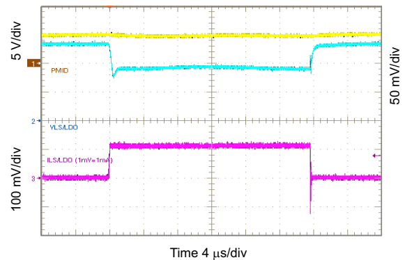
Figure 10-54. 1.8 V_{\text{LSLDO}} Load Transient, 0 to 100 mA
