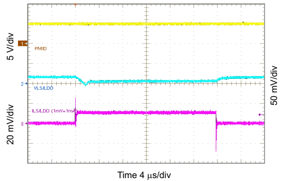
Figure 10-48. 1.2 V_{LSLDO} Load Transient, 0 to 10 mA
