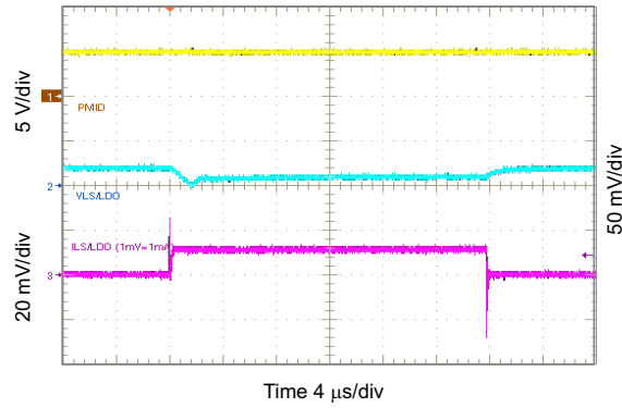
Figure 10-51. 3.3 V_{\text{LSLDO}} Load Transient, 0 to 10 mA
