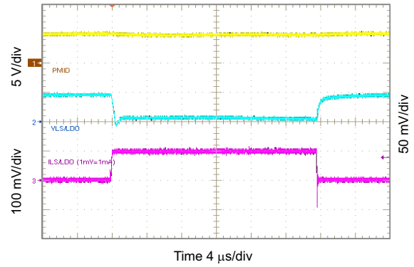
Figure 10-52. 0.8 V_{\text{LSLDO}} Load Transient, 0 to 100 mA
