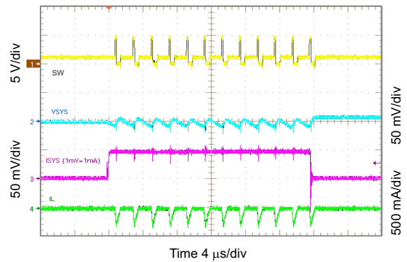
Figure 10-31. Light Load Operation Showing SW
