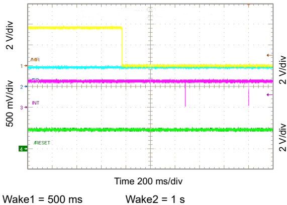
Figure 10-63. Show \overline{MR} Timing
