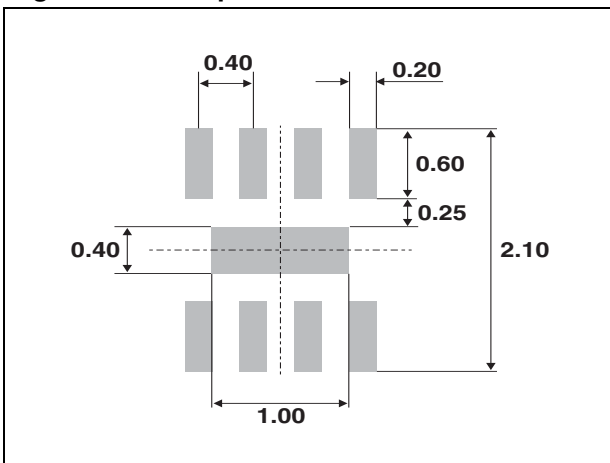
Figure 9. Footprint
