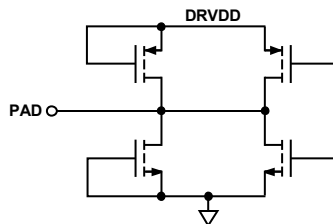
Figure 55. Digital Output
