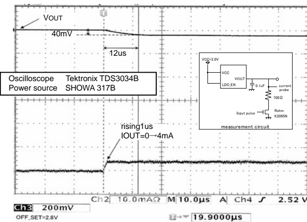
BU9829GUL-W Evaluation result (IOUT=0mA→4mA, COUT=1.0µF) Figure 56. CL=1.0µF Transitional response
