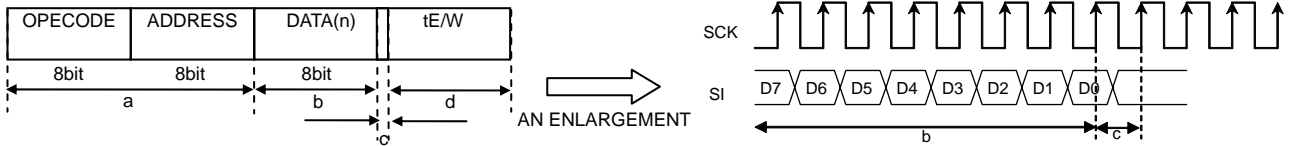
Figure 41. WRITE, PAGE_WRITE, VSET_WRITE READ VSET_READ Cancel Timing
