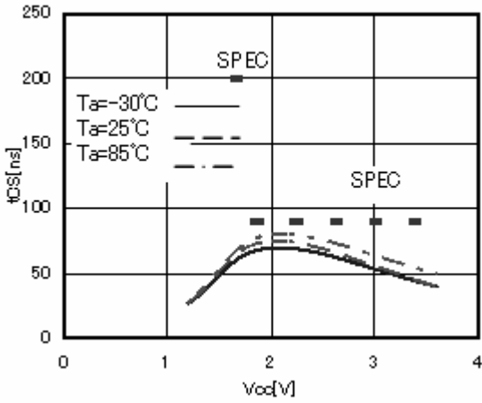
Figure 17. CSB high time tCS
